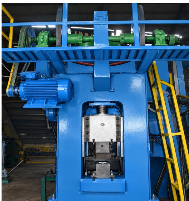
Hot Forging
